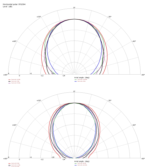
HORIZONTAL 1/3 OCTAVE POLAR PLOTS
