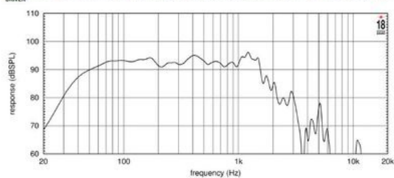
FREQUENCY RESPONSE MADE IN 170 LT. ENCLOSURE TUNED AT 34 Hz IN FREE FIELD (H) ENVIRONMENT. ENCLOSURE CLOSES THE REAR OF THE DRIVER
