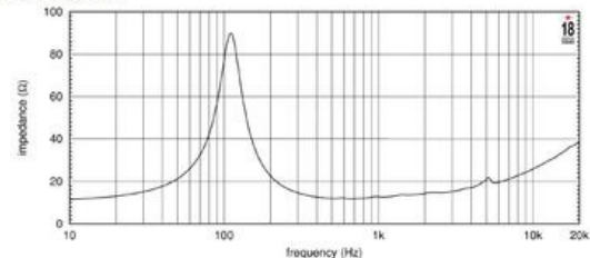
FREE AIR IMPEDANCE CURVE
