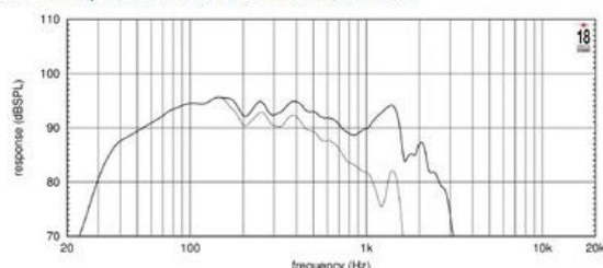
FREQUENCY RESPONSE MADE IN 200 L.T. ENCLOSURE TUNED AT 20 Hz IN FREE FIELD (H) ENVIRONMENT. ENCLOSURE CLOSES THE REAR OF THE DRIVER, THE THIN LINE REPRESENTS AS DED. OFF AXIS FREQUENCY RESPONSE
